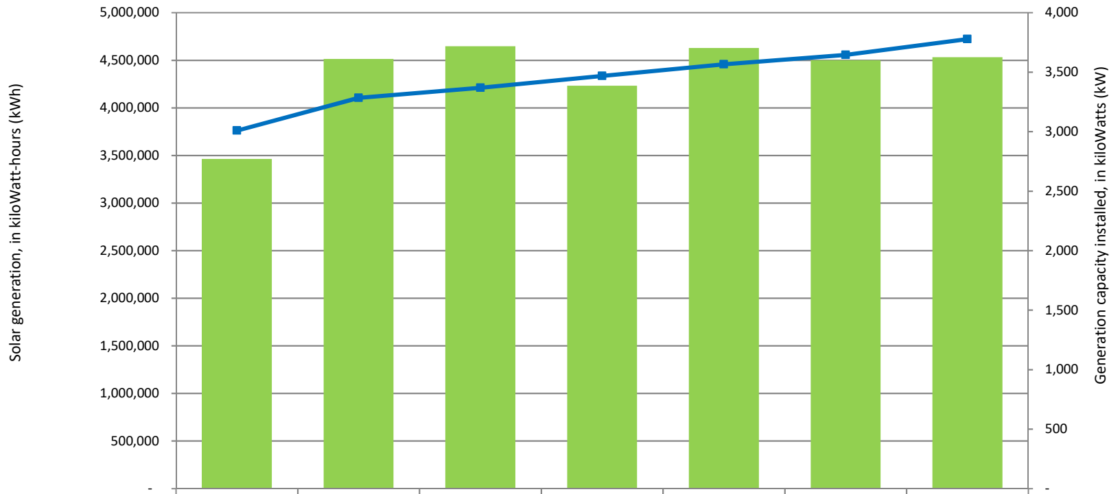
Annual Solar Power Generated by Green Power Providers Participants in Shelby County
